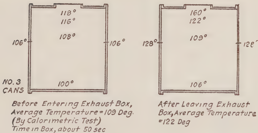
FIG. 3 TEMPERATURES ATTAINED IN EXHAUST BOX
